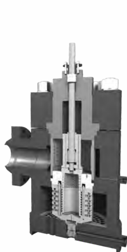
Valve with Zick Twist & De-Laval Nozzle
