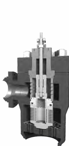
Valve with Zick Twist Cage
