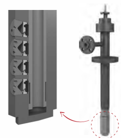
IC Desuperheater
