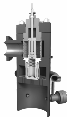
Valve with Zick Twist Cage and SL Nozzle
