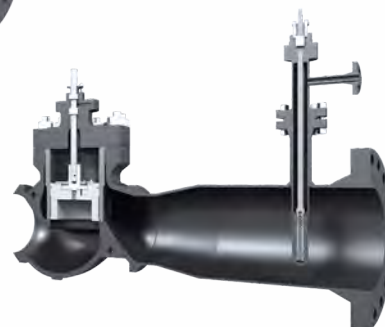
Valve with IC DSH
